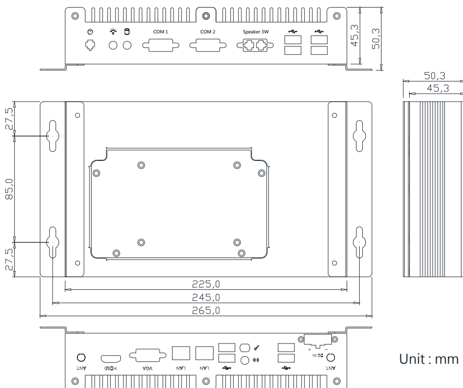
AES-2210D-C2-M8-HG5SP1
